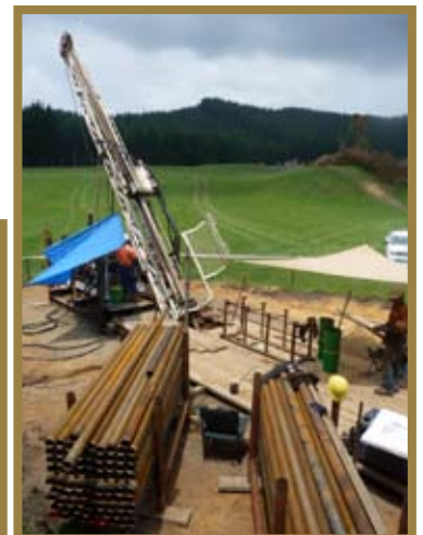
Drilling at Muirs, December 2010
