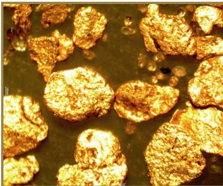
Fine grained gold from bulk testing within the Manuherikia Valley, Central Otago
