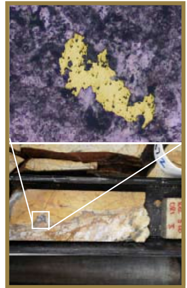
Below: Silicified core from WKP, with a close up of gold in-situ, top
